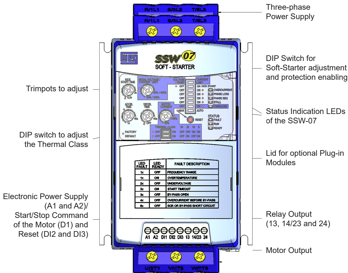
Figure 2.1 - Frontal view of the SSW-07
