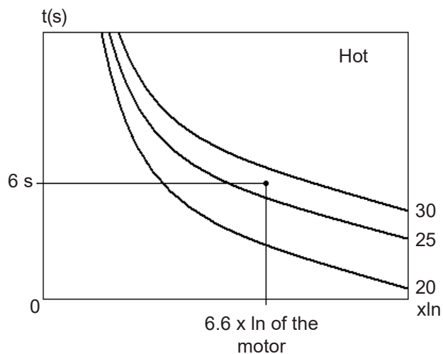
Figure 5.11 - Checking the maximum class of curves in hot condition
