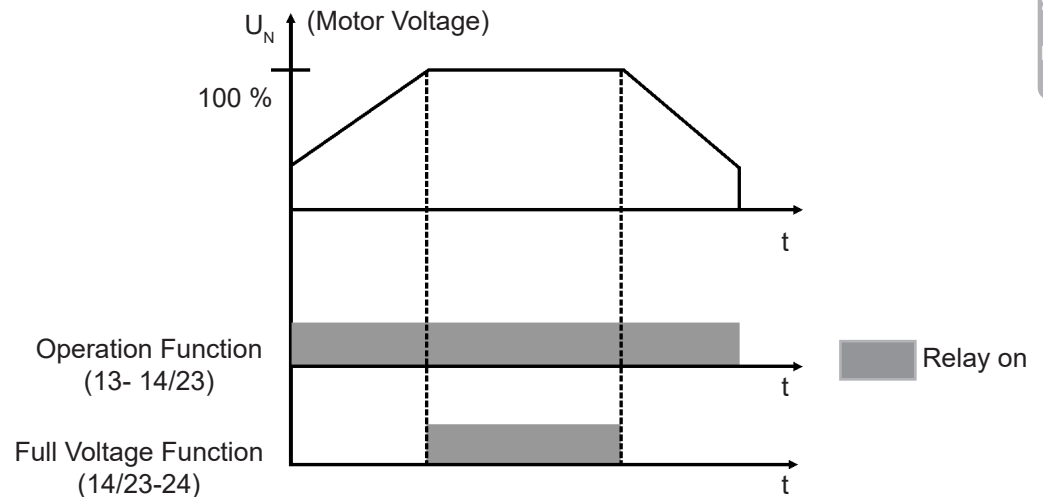
Figure 4.11 - Output relay operation
