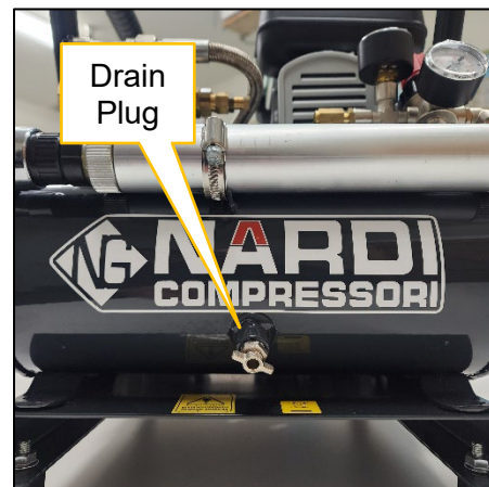
Figure 8. Air tank drain plug.
