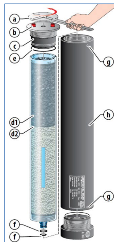
Figure 6. Filter cartridge and cartridge parts.
