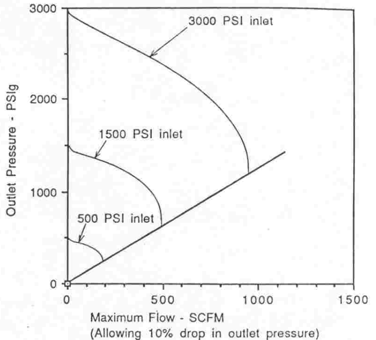
MODEL 873 SERIES FLOW CHART
