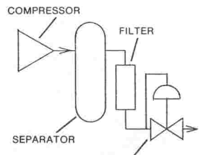
MODEL 635 BACK PRESSURE REGULATOR MAINTAINS PRESSURE IN FILTER AND SEPARATOR
